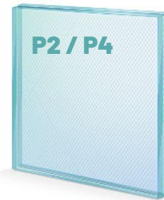
P2 2x4mm + 2 layers of foil P4 2x4mm + 4 layers of foil
